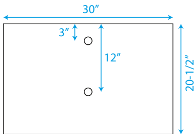
TOP VIEW OF VANITY CABINET
