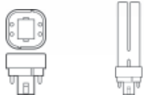
G24q-3 L-PLC26W/27 Base 26W G24q-3 Base
