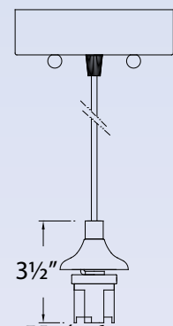
V2426 1x26W G24q-3 Base 120V/277V HPF Electronic Ballast
