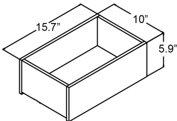
Drawer
