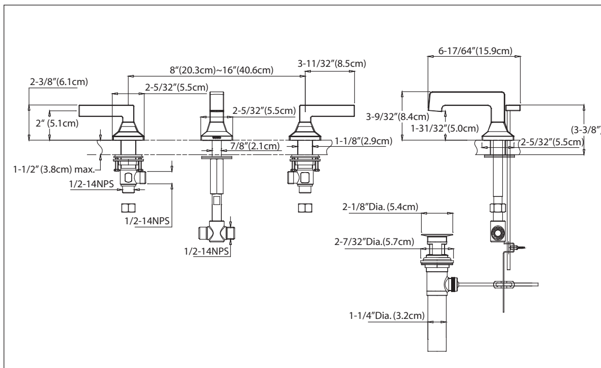
TL930DD - Lloyd™ Widespread Lavatory Faucet
