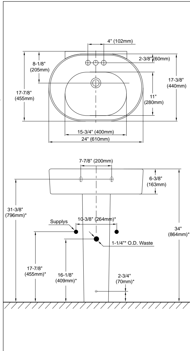
LPT790 Nexus™ Pedestal Lavatory
