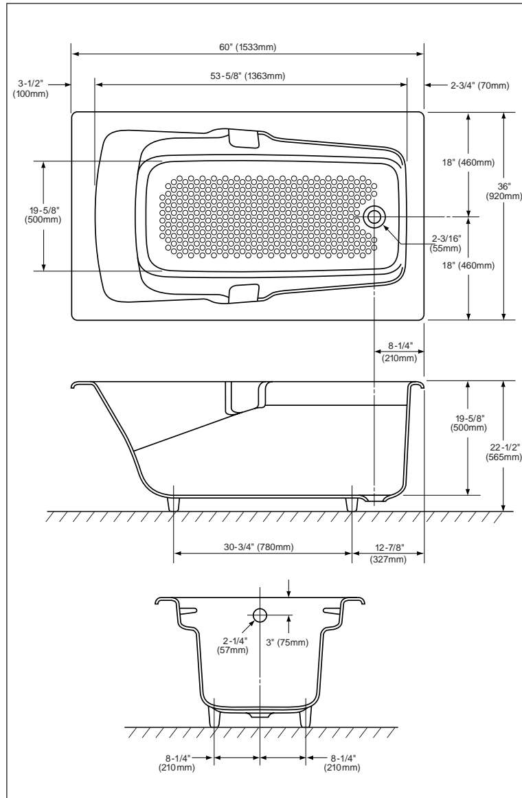
FBY1500P - Cast Iron Bathtub
