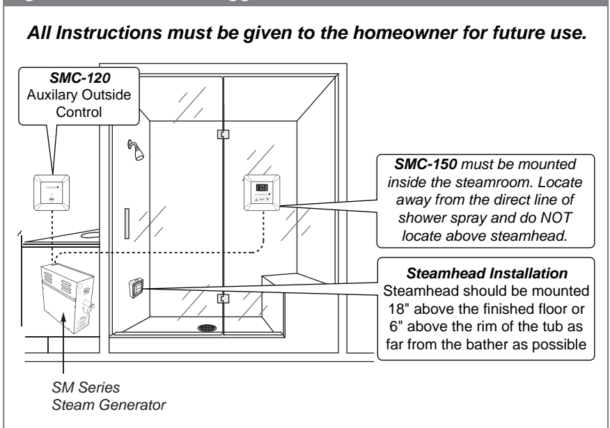
Figure 4 - Installation Suggestions
