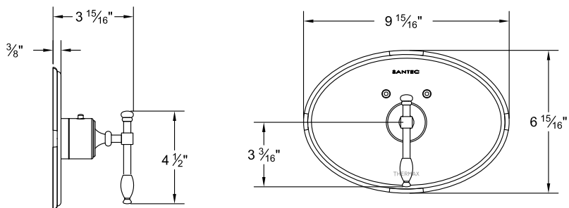
7093LV__-TM Thermax Thermostatic Control Trim
