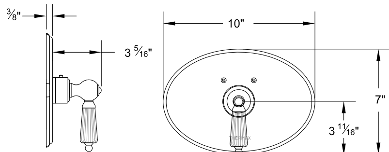
7093LL_-TM Thermax Thermostatic Control Trim
