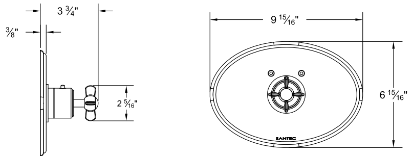
7093ET__-TM Thermax Thermostatic Control Trim
