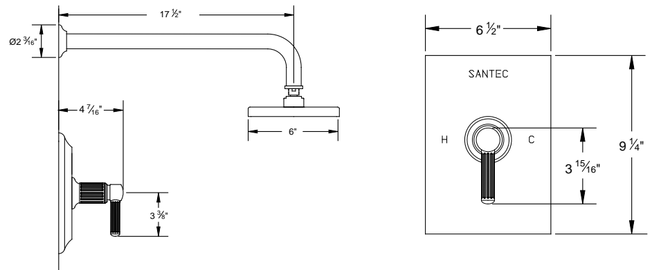
7093EN__-TM Thermax Thermostatic Control Trim
