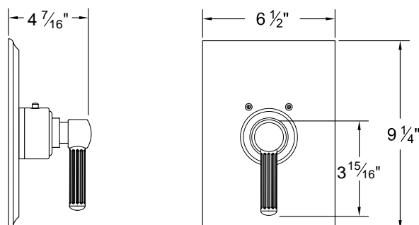
7093EN__-TM Thermax Thermostatic Control Trim
