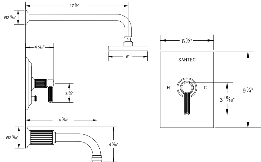
3632EN__-TM Pressure Balanced Shower Trim Set
