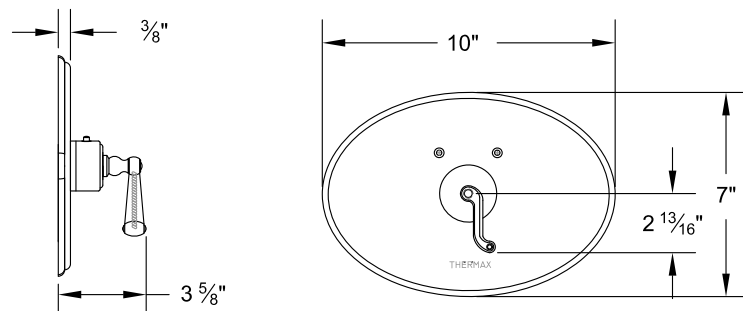
7093AA__-TM Thermax Thermostatic Control Trim
