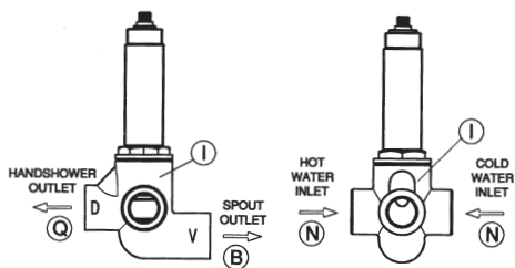
DIVERTER CONNECTIONS
