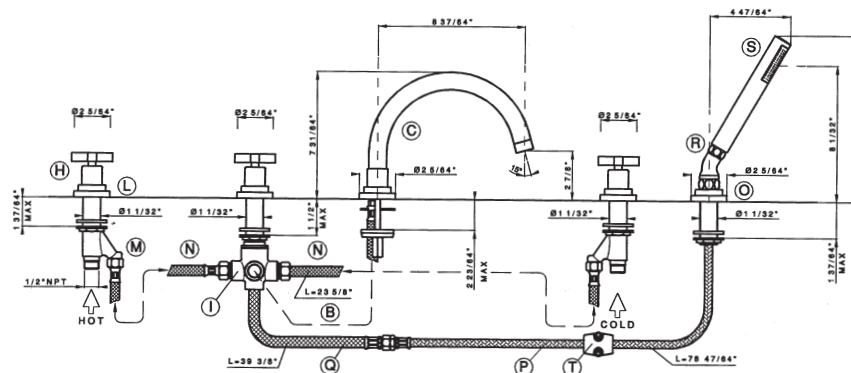
DIVERTER CONNECTIONS
