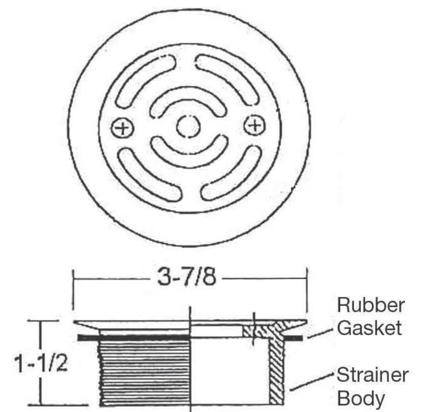
Strainer
