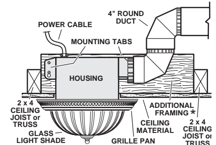
HOUSING MOUNTED TO 2x4 TRUSS
