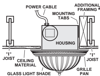
HOUSING MOUNTED TO "1" JOIST
