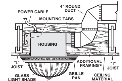
HOUSING MOUNTED TO "1" JOIST
