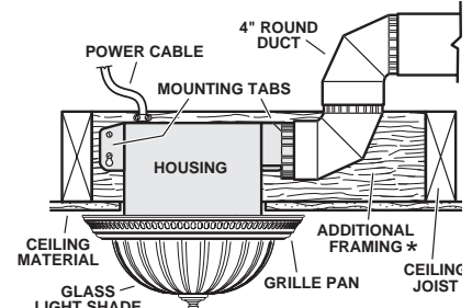
HOUSING MOUNTED TO ADDITIONAL FRAMING
