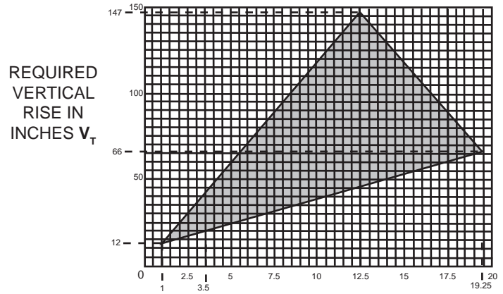
HORIZONTAL VENT RUN PLUS OFFSET IN FEET H_T The shaded area within the lines represents acceptable values for H_T and V_T
