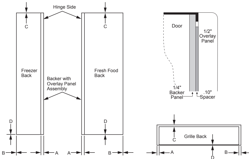
PANEL DIMENSIONS
