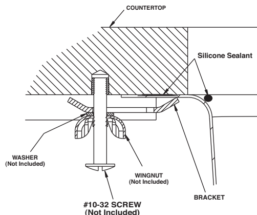
Installation Detail
