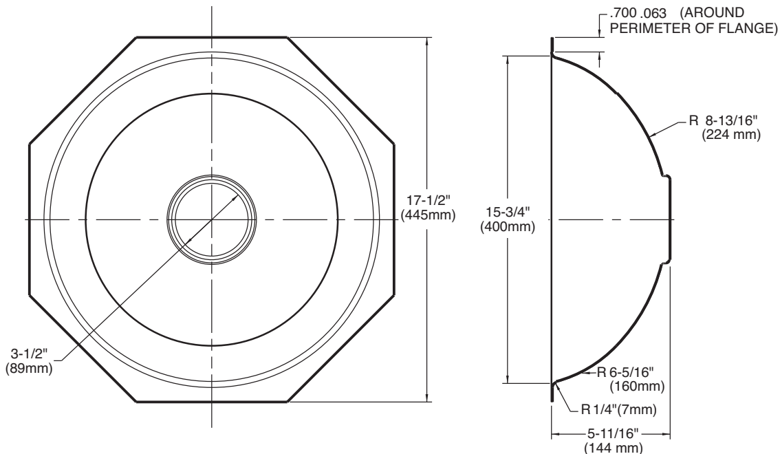
Installation Detail
