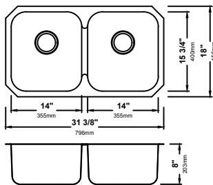
KBU29 31 3/8" x 18" x 8" Min Cabinet Size: 36" Matching Grid: KBG-29 (2) Drain Model #: BST-1 & ST-1 (2)
