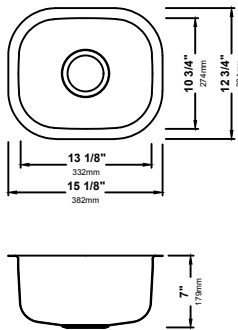
KBU17 15 1/8" x 12 3/4" x 7" Min Cabinet Size: 18" Drain Model #: ST-1
