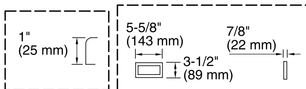
Drop-in Rim Detail
