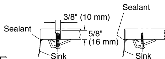
Marble-slab Installation
