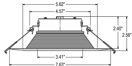
WF6
