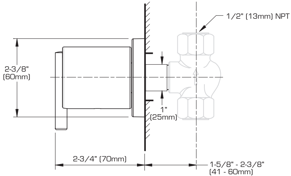
1/2" (13mm) NPT VALVE
