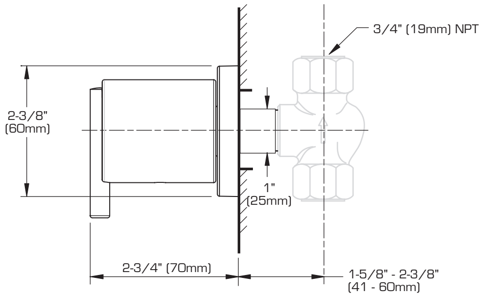
3/4" (19mm) NPT VALVE
