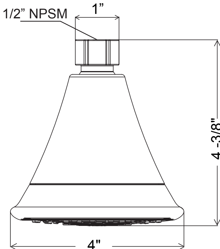
INSTALLATION DIMENSIONS
