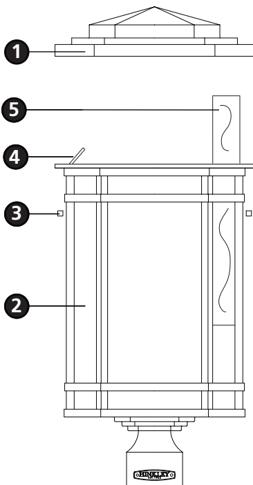
Drawing 2 - Lamping Instructions
