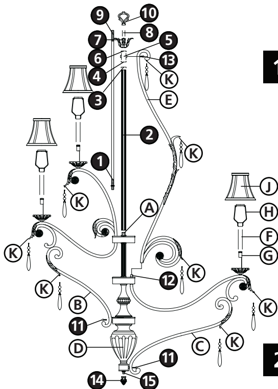
Drawing 1 - Fixture Assembly
