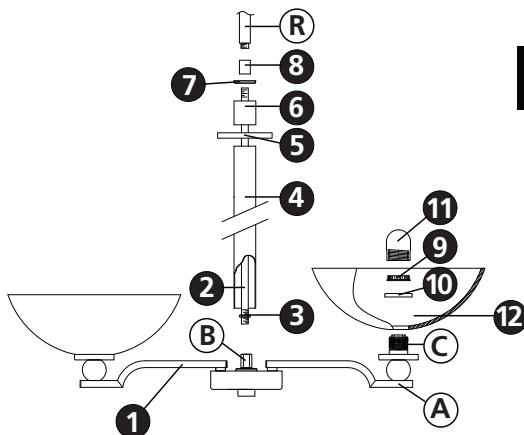
Drawing 2 - Fixture Assembly
