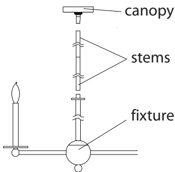
Drawing 3 - Stem Assembly
