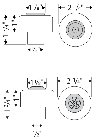
Body Jet 06889XX0 Body Jet - Spray 06342XX0
