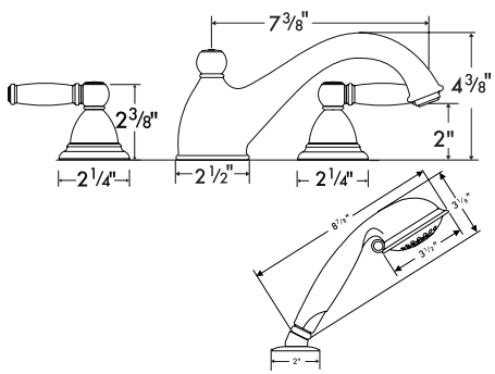
Limbo - Lever handles shown
