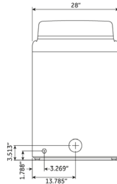
REAR VIEW
