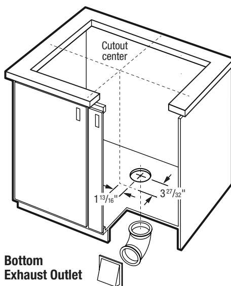
Alternate Duct Transition Kit
