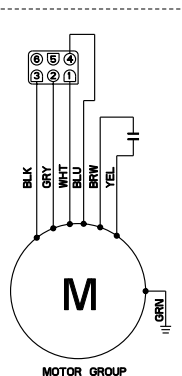
MOTOR GROUP
