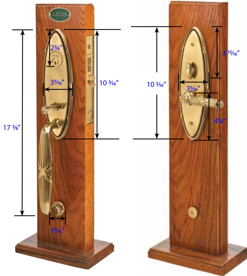
Oval Ribbon & Reed Trim Style Part # UL 3342
