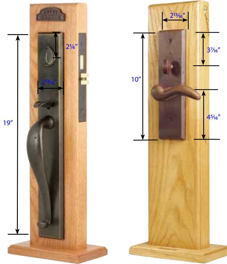
Rectangular Full Length UL Mortise Part # UL 3326
