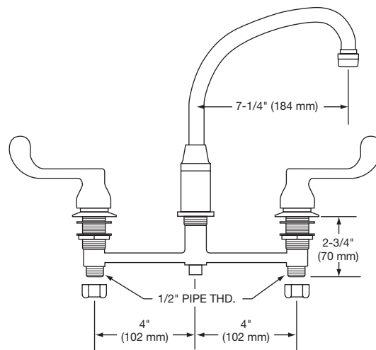
LKDC2432BH Illustrated
