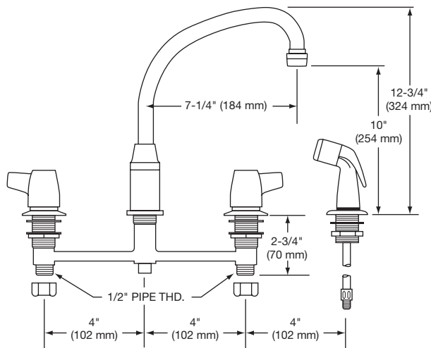
LKDC2433 Illustrated
