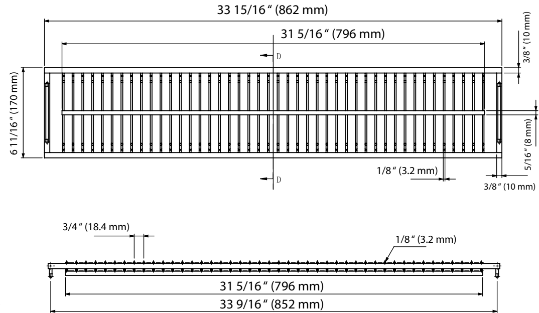
Warming Rack
