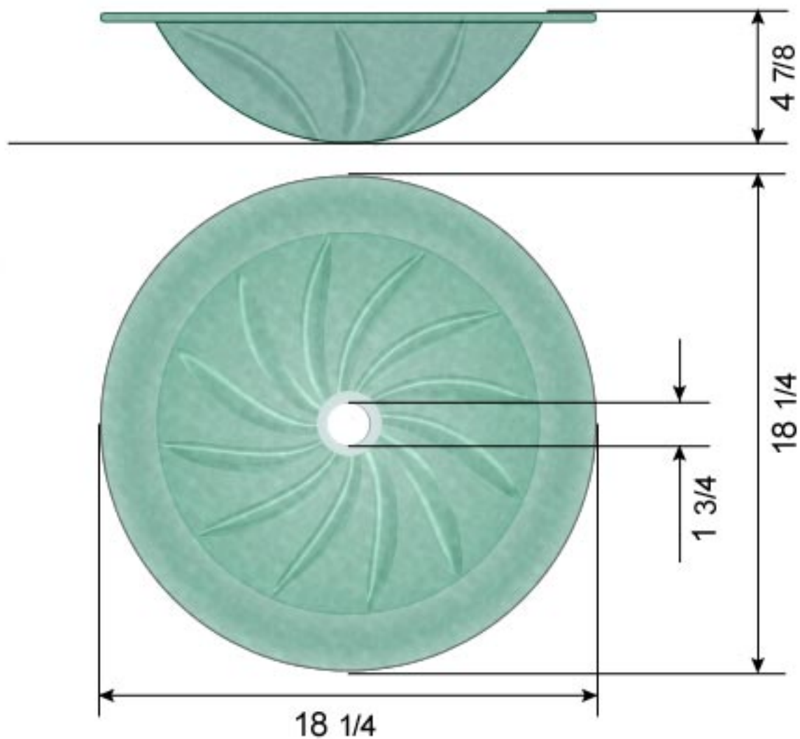
DLBG-19C with optional Faucet FVDL-711
