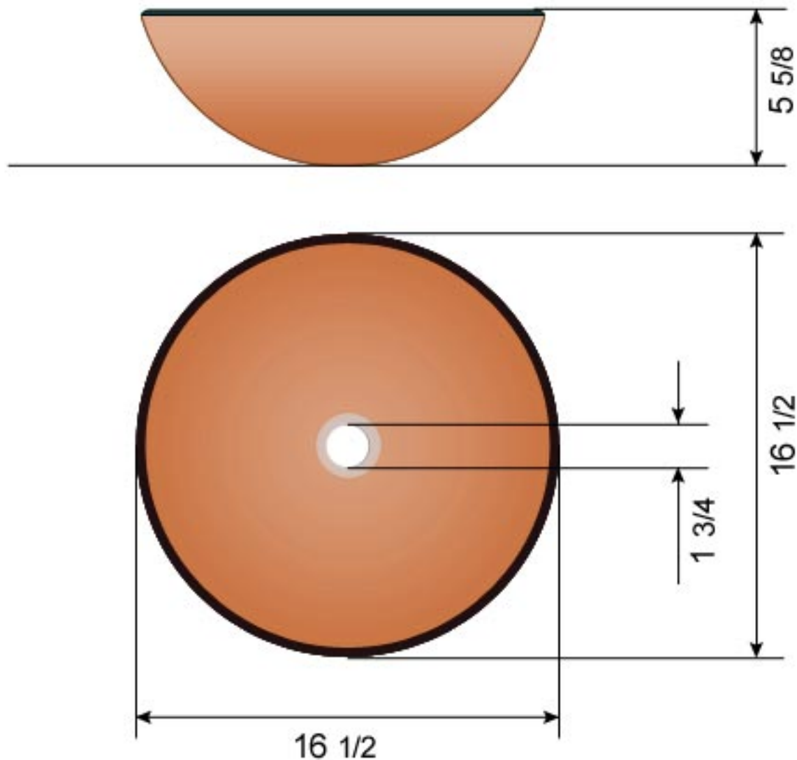
DLBG-08R with optional Faucet FVDL-711R
