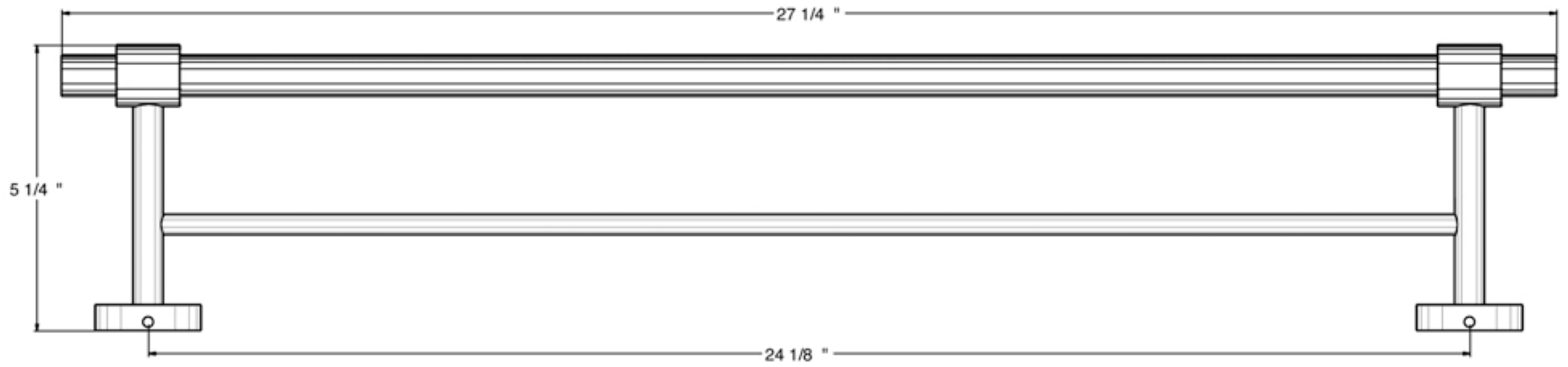
FRONT VIEW
