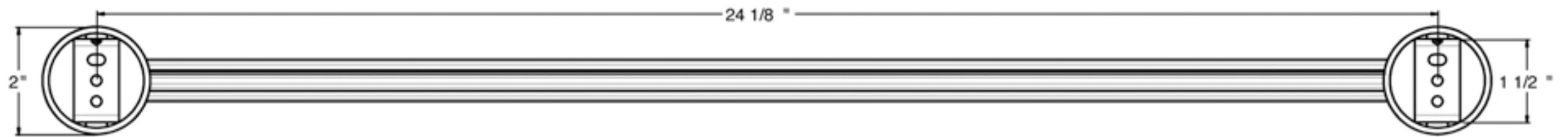
BOTTOM VIEW
