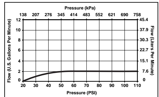
R2900-MIX Pressure and Flow Guidelines
