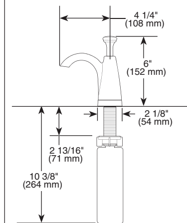
Optional Soap Dispenser RP47888
