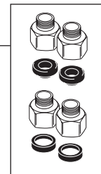
RP63263 Adapters 3/8"-24 UNEF to 1/2"-20 UN & 3/8"-24 UNEF to 1/2"-14 NPSM Adaptadors 3/8"-24 UNEF to 1/2"-20 UN & 3/8"-24 UNEF to 1/2"-14 NPSM Adaptateurs 3/8 po-24 UNEF to 1/2 po-20 UN et 3/8 po-24 UNEF to 1/2 po-14 NPSM
