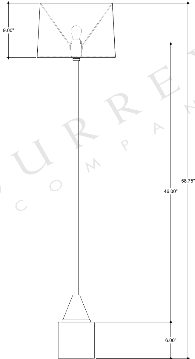
FRONT VIEW
