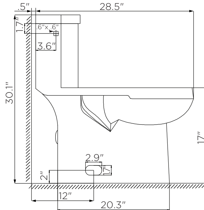
SIDE VIEW
