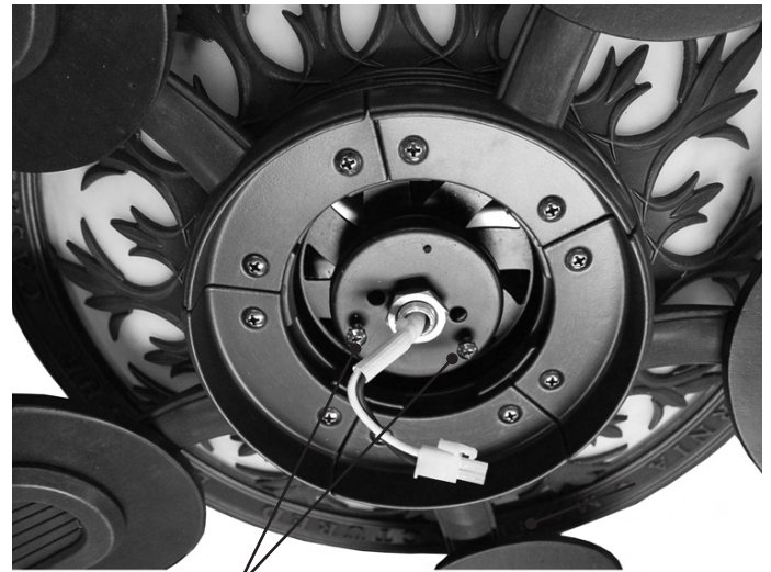
Light adapter screws (2)
