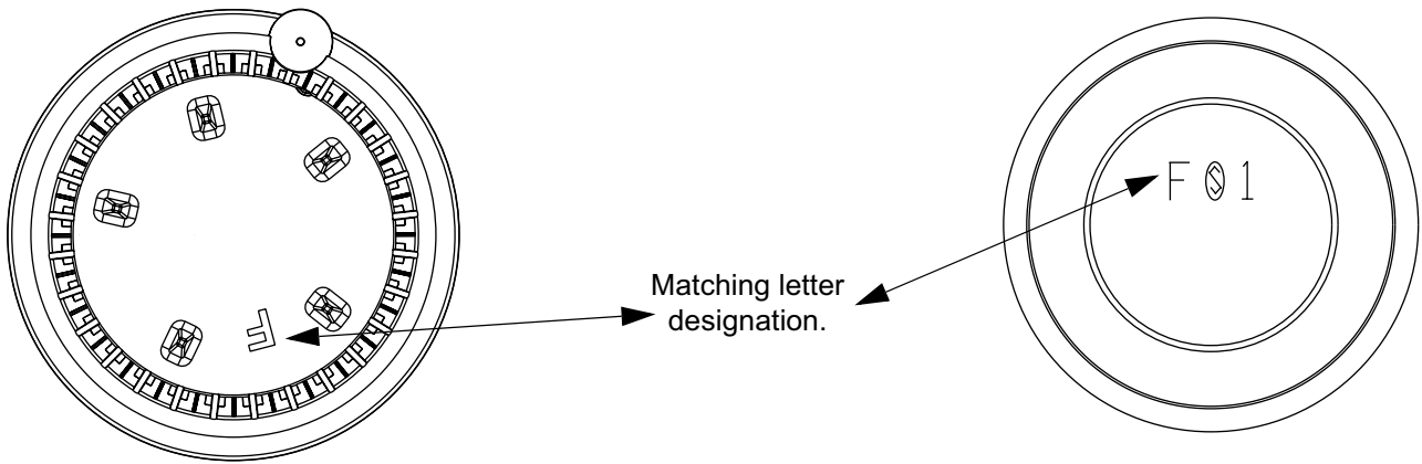
Figure 4: Burners Caps
