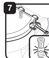
7 As you hold seat centered on bowl, tighten lower section of STA-TITE® nuts until they snap off
