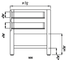
SIDE
