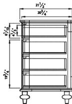
SIDE
